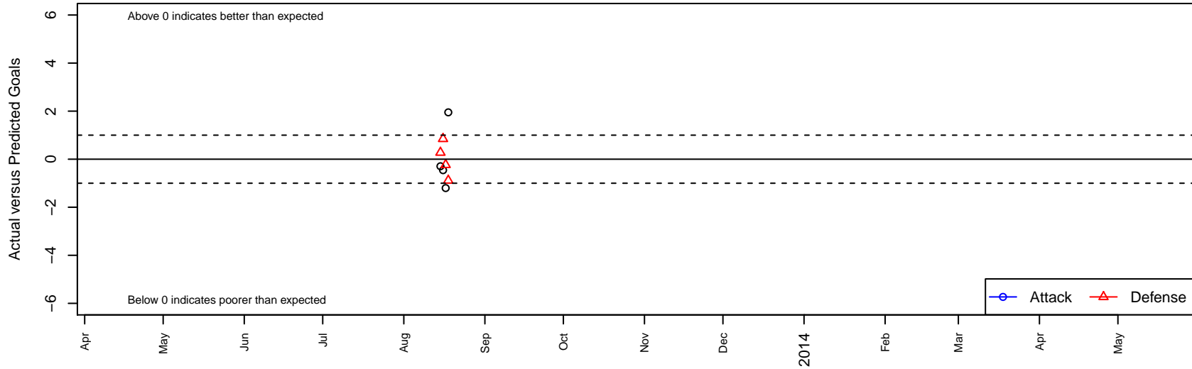
Watermelons B97 Dots are actual minus expected GF (blue circles) and GA (red triangles). Blue line is smoothed change in attack strength. Red is smoothed change in defense strength.
